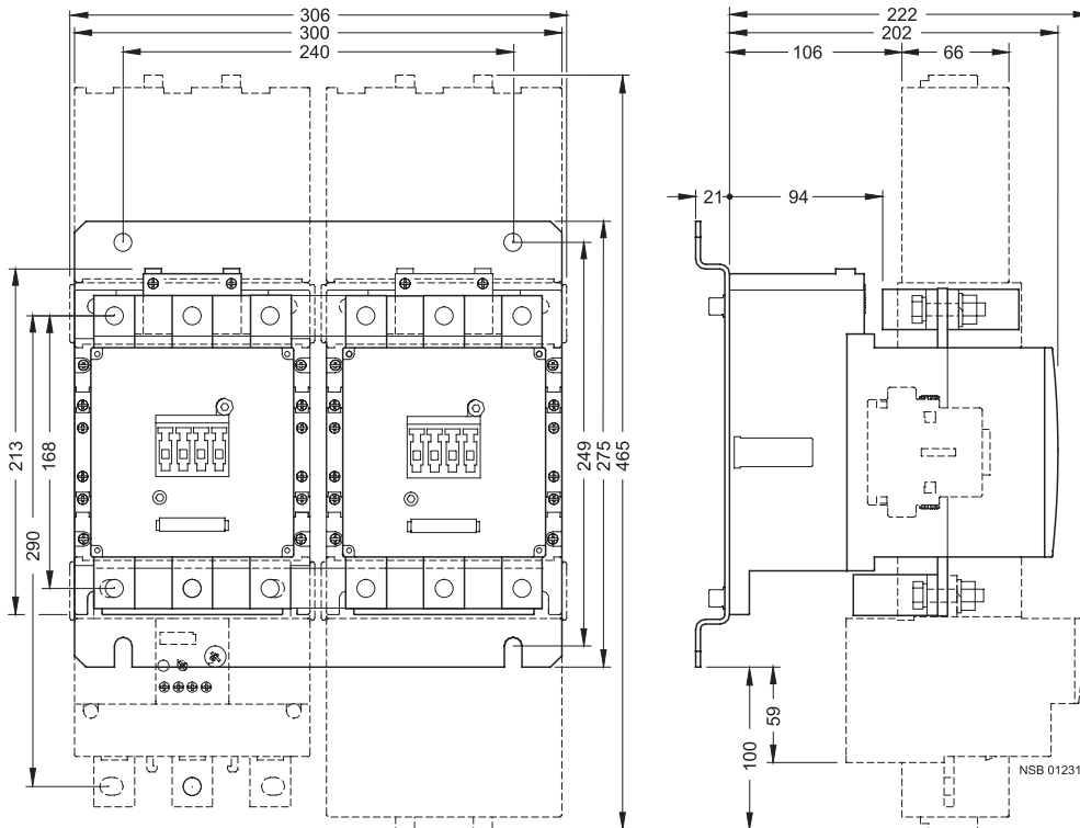
Size S10
