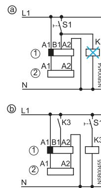
Time-delay block Contactor
