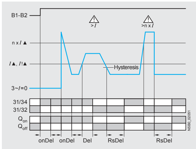
Current overshoot
