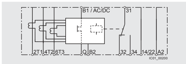
3RR2241-1F.30
