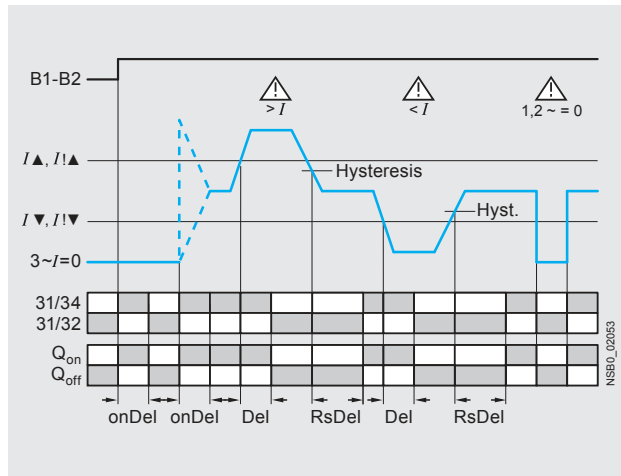
Range monitoring
